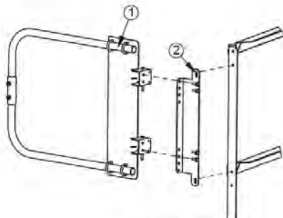
HINGED LEFT
