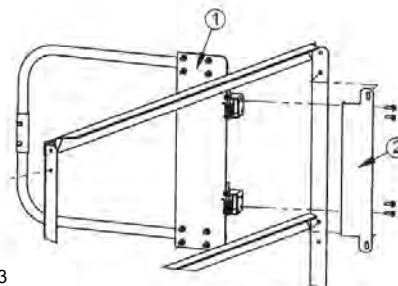
HINGED RIGHT
