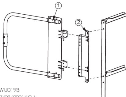
HINGED LEFT
