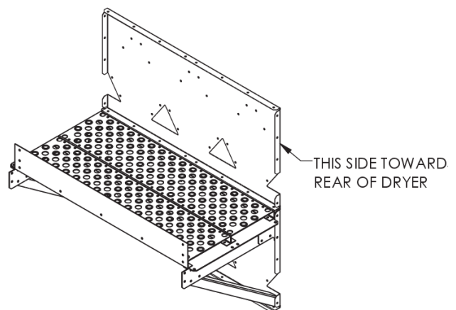
Fig. 11 – Attaching planks
